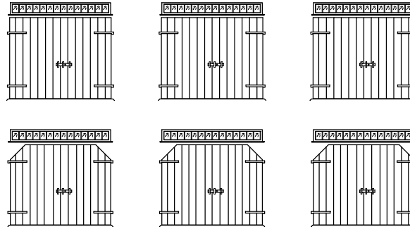
9' Swing-out Doors and Transoms
