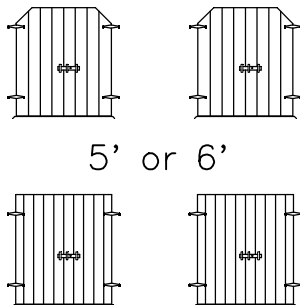
Swing-out Doors
